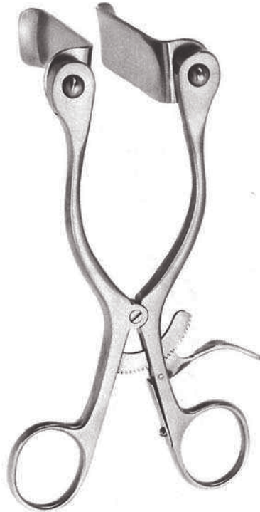
CASPAR 18.720.00 compl. 18.720.15 ohne Valven · without blades sans valves · sin valvas · senza valve
